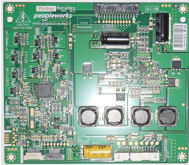
PPW-LE42GD-O (A) REV0.5 LG 42LW450U LED DRIVER BOARD 130.00TL
